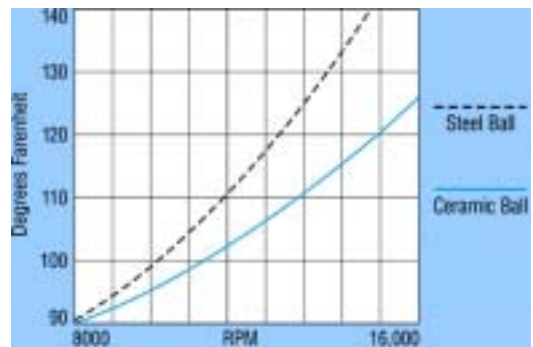
As running speed increases, ceramic balls run cooler than conventional steel balls. The reduced heat build-up prolongs lubricant life.
