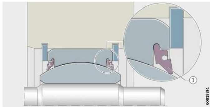
1: Example of Lip Seal
